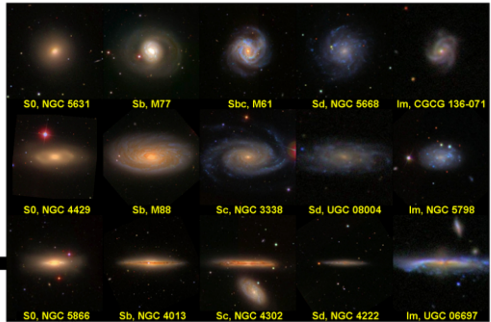
Normal Lenticular (S0), Spiral (S), and Irregular (Im) galaxies
