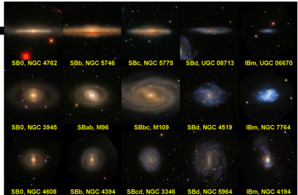
Barred Lenticular (SB0), Spiral (SB), and Irregular (IBm) galaxies
