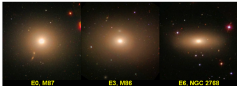
Elliptical (E) galaxies
